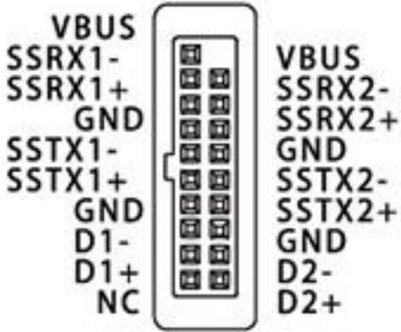
USB 3.0
