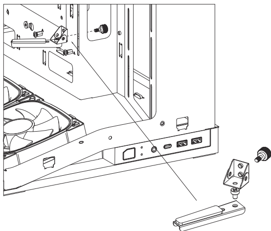
Graphics card holder
