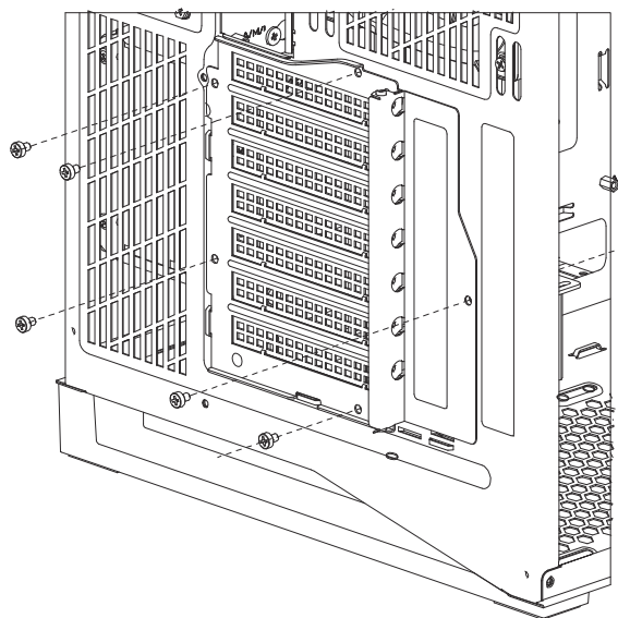
Horizontal graphics card
