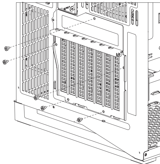
Vertical mounted graphics card
