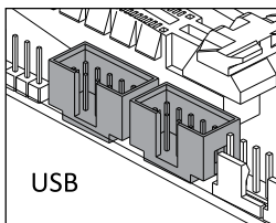
9-pin USB 2.0 connector
