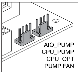
Motherboard
